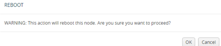
Figure 25 Reboot Dialog
